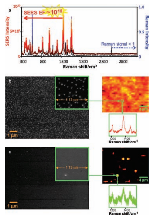
Figure 2. Raman and SERS spectra at hot spots. (a) Bulk Raman spectrum of 15NAT molecules in aqueous solution (right scale), compared to the SERS spectrum of the same molecules recorded by using the scheme of Figure 1a with nanostars (left scale). The 1OT:15NAT ratio is 100:1. The nanostar-assisted SERS signal per molecule is \sim 10^{10} times larger than the Raman signal per molecule (enhancement factor EF \sim 10^{10} ). (b) Left: SEM images showing bound nanoparticles with a density of 27 \pm 7 particles per \mu\text{m}^2 . Right: SERS spatial mapping over the highlighted region in the SEM image. (c) Single-particle SERS mapping recorded from a sample with less than 1 particle per \mu\text{m}^2 . Details of SERS spectra collected within an area of 1.28\ \mu\text{m}^2 are shown for the samples in images b and c.
